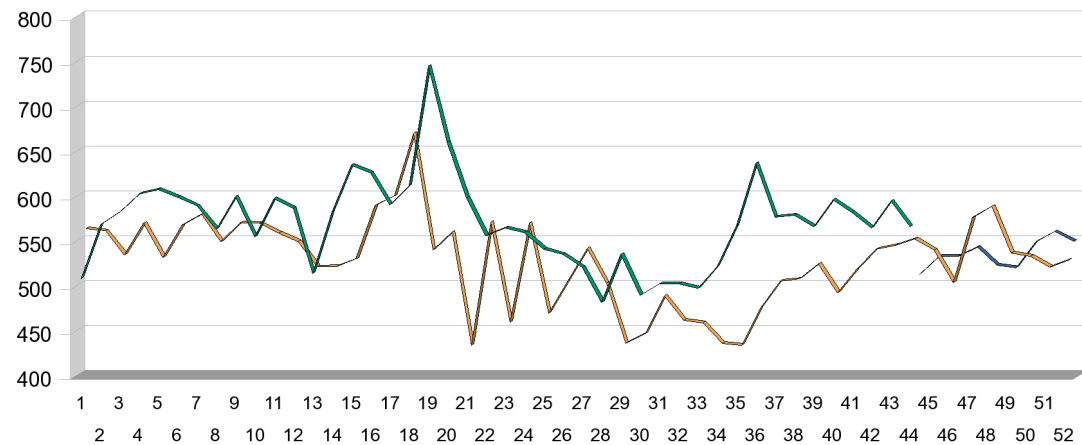
Totalkväve, µg/L
